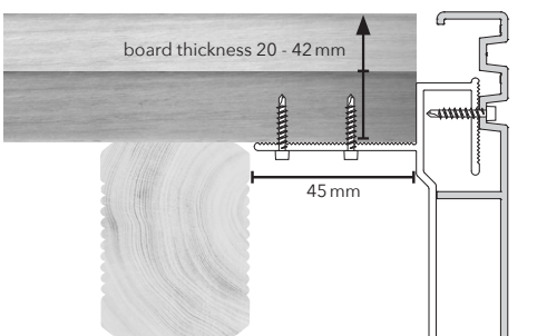
RELO VH is pre-mounted to the deck board RELO V and RELO VH can be cut to length
