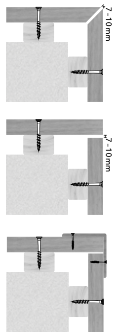
Eckanschlüsse
